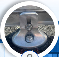
Roof Penetration
